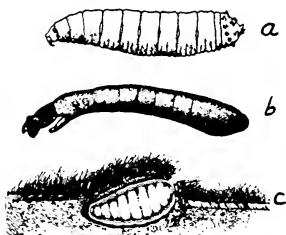
Fig. 28. Larvae: a, cabbage root maggot, Hylemyio brassicae (Bouche); b, buffalognat, Simulium pecuarum Riley; c, common cattle grub, Hypoderma lineatum (De Villiers) under host skin. (U.S.D.A.)
